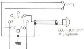
3. External microphone
