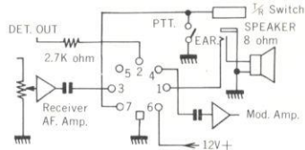
6. Internal connection
